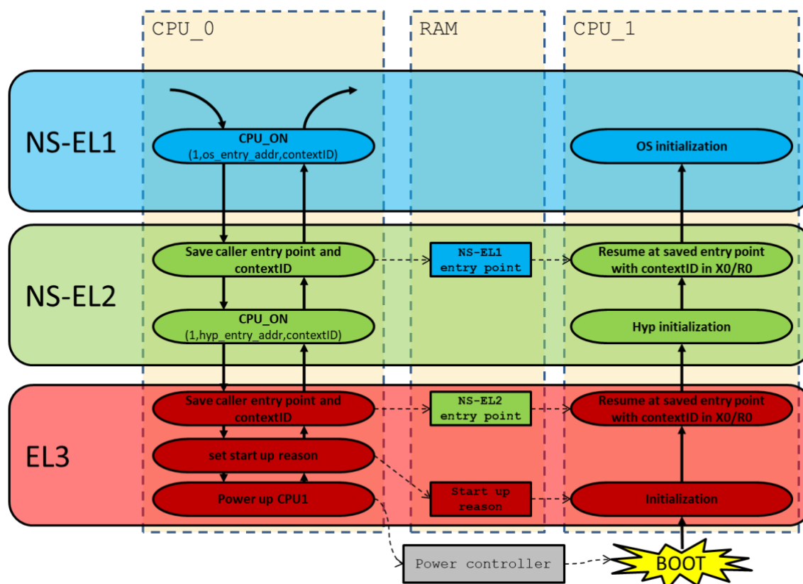
Figure 7 Example call flow for a CPU OFF call
