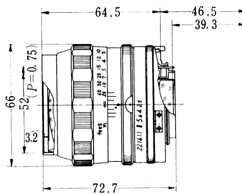
Dimensions of Nikkor-P Auto 1:2.5 f=105\text{mm} .
