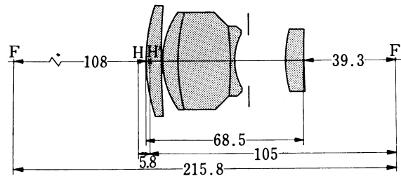
Optical formula of Nikkor-P Auto 1:2.5 f=105\text{mm} .
