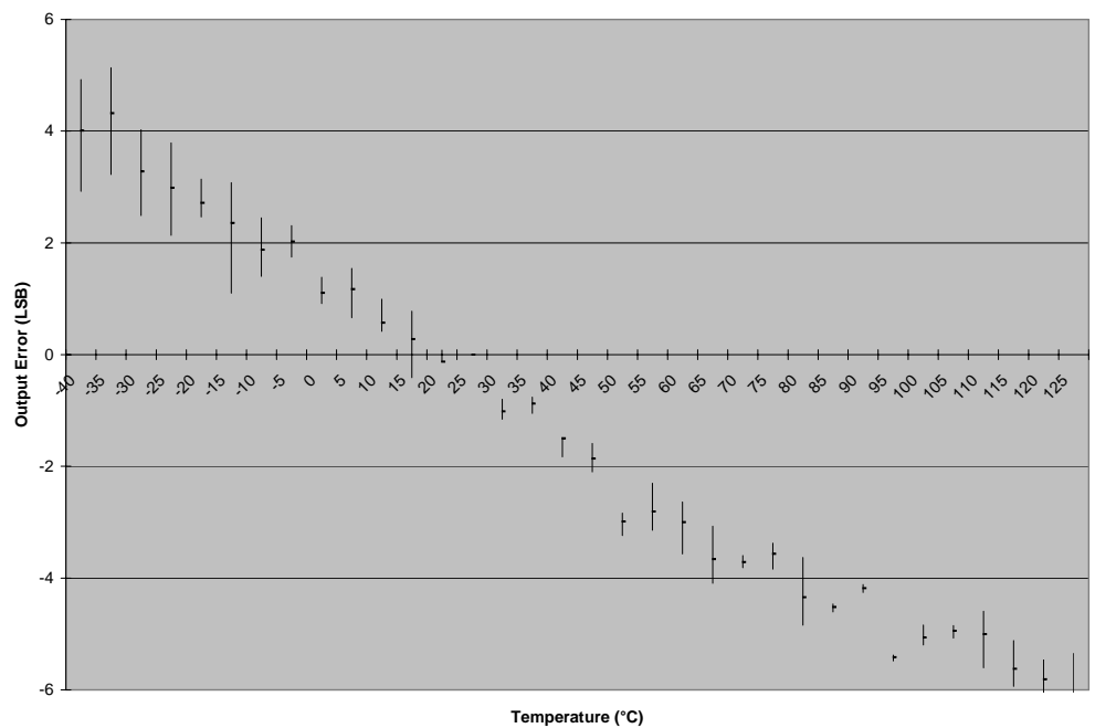
Figure 3-8. Two-point compensated with T_2 5^\circ\text{C} above ideal value.
