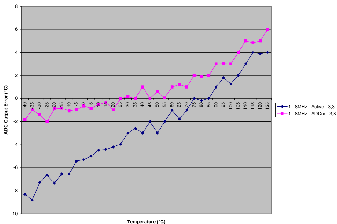
Figure 3-2. ADC output error at 8MHz CPU frequency, 3.3V.
