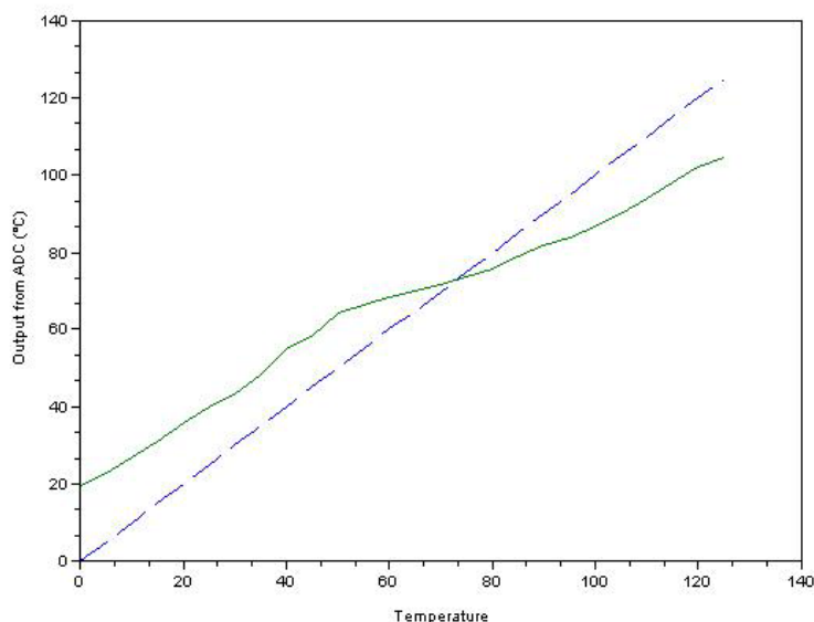
Figure 2-1. ADC and ideal output.
