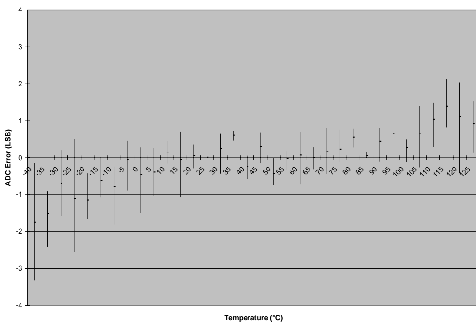
Figure 3-7. ADC output error in active mode, 8MHz, 3.3V, two-point compensated.
