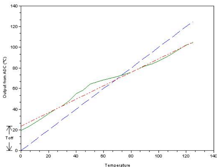
Figure 2-2. ADC output with line defined by calibration points.
