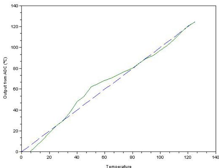
Figure 2-4. ADC output with offset and gain errors removed.
