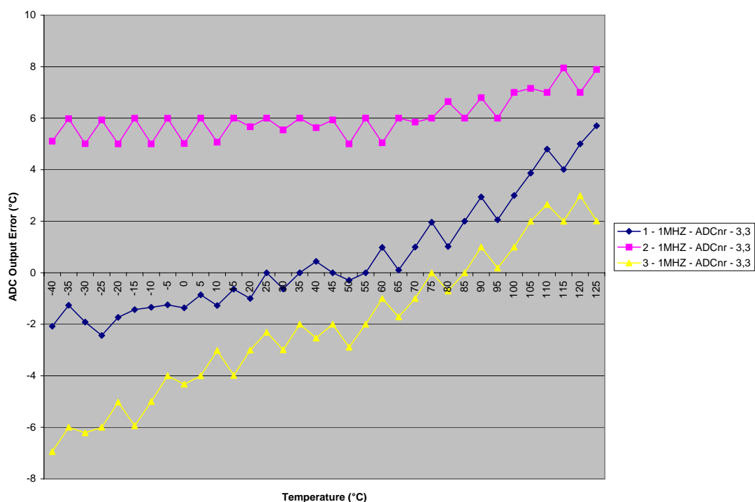
Figure 3-6. ADC output error, ADC Noise Reduction Mode, 1MHz, 3.3V, no compensation.
