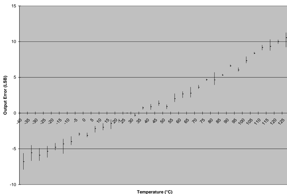
Figure 3-9. Two-point compensated with T_2 5°C below ideal value.
