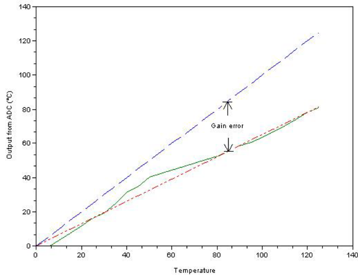
Figure 2-3. ADC output with offset error removed.
