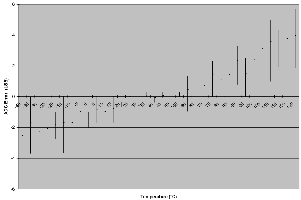
Figure 3-3. ADC output error in ADC Noise Reduction Mode, 1MHz, 3.3V, offset compensated.
