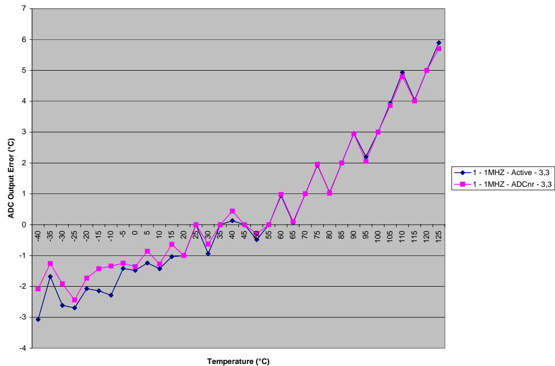
Figure 3-1. ADC output error at 1MHz CPU frequency, 3.3V.
