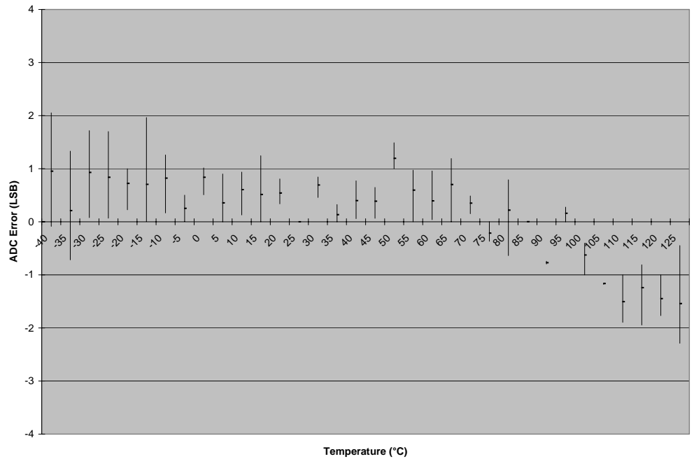
Figure 3-5. ADC output error in ADC Noise Reduction Mode, 1MHz, 3.3V, two-point compensated.
