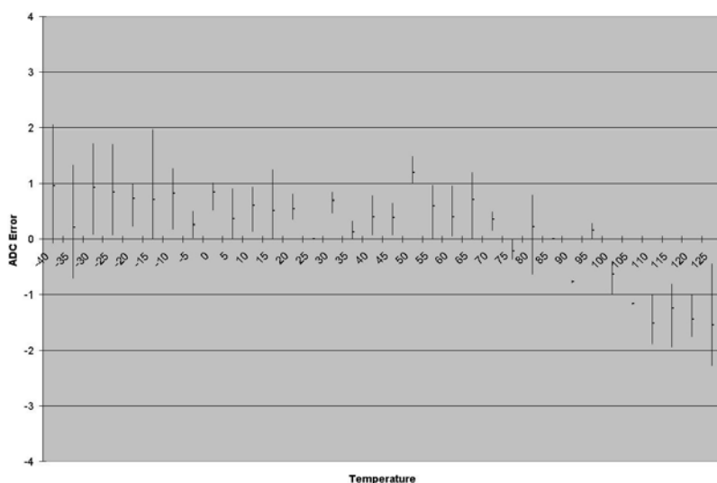
Figure 1-1. ADC output error in ADC Noise Reduction Mode, two-point calibrated.
