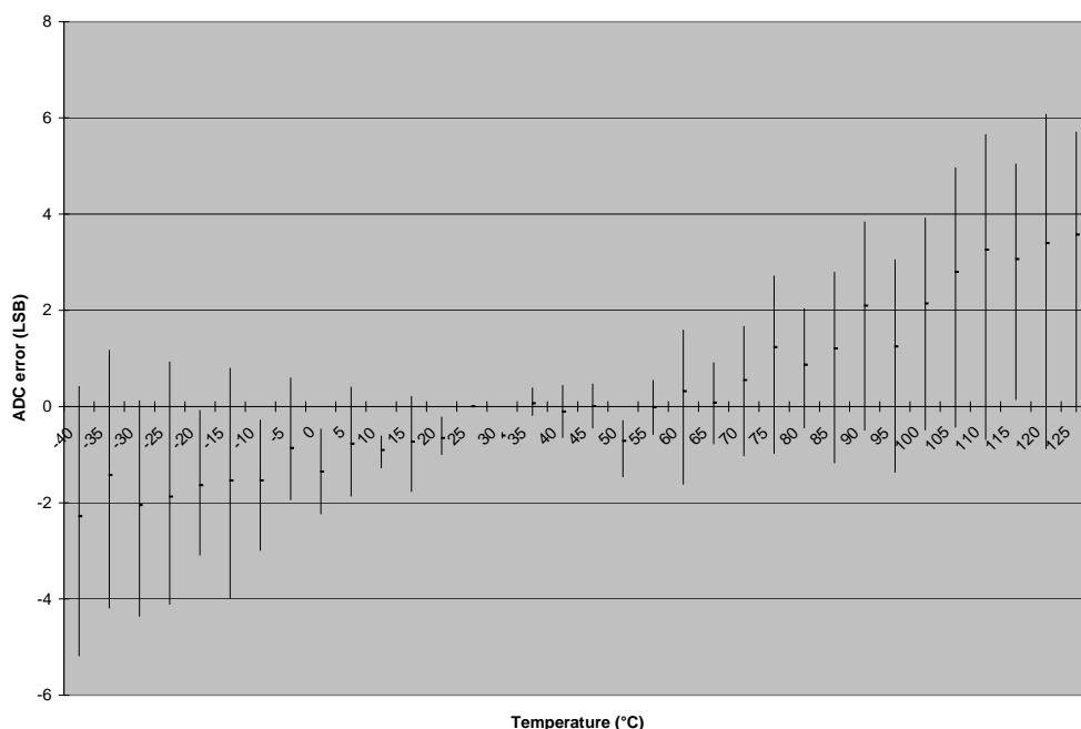
Figure 3-4. ADC output error in ADC Noise Reduction Mode, 1MHz, 3.3V, gain compensated.
