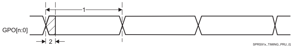
Figure 7-92. PRU-ICSS PRU Direct Output Timing
