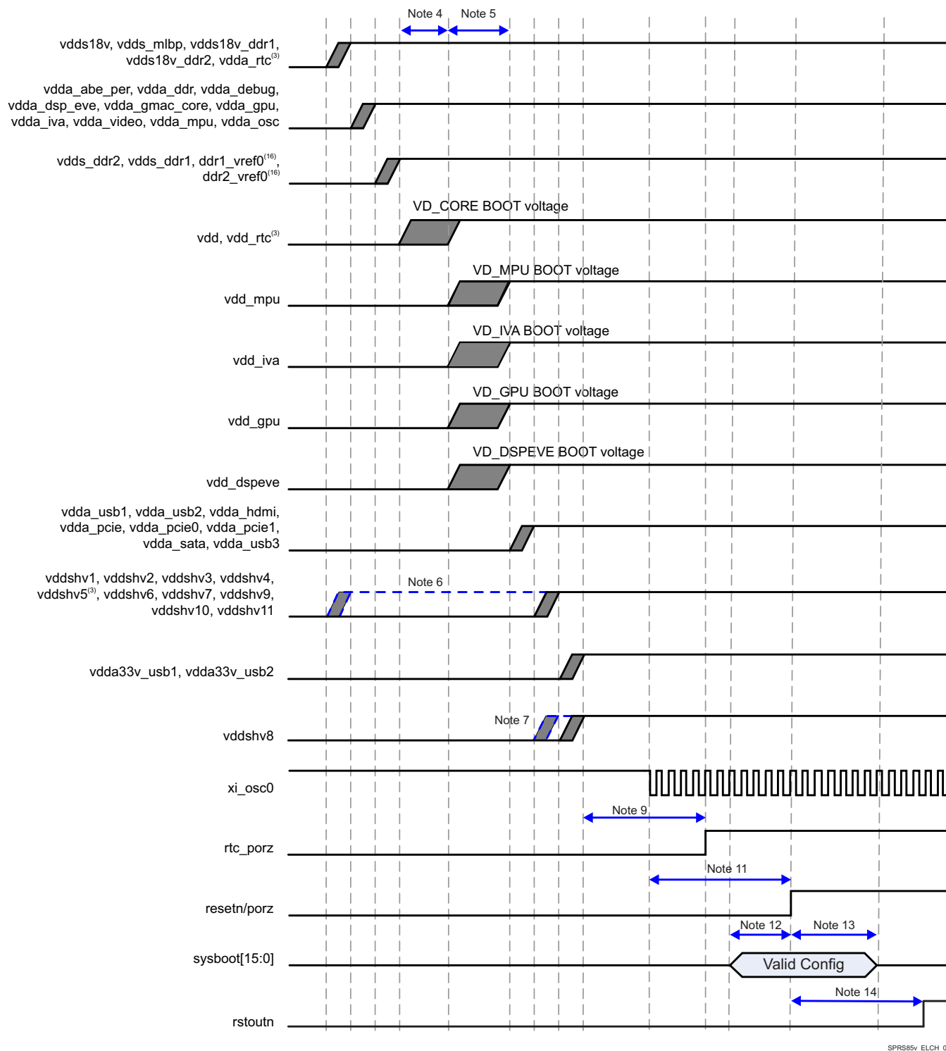
Figure 5-2. Power-Up Sequencing
