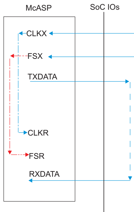
Figure 7-49. McASP1-8 CI-FI- – SYNC Mode
