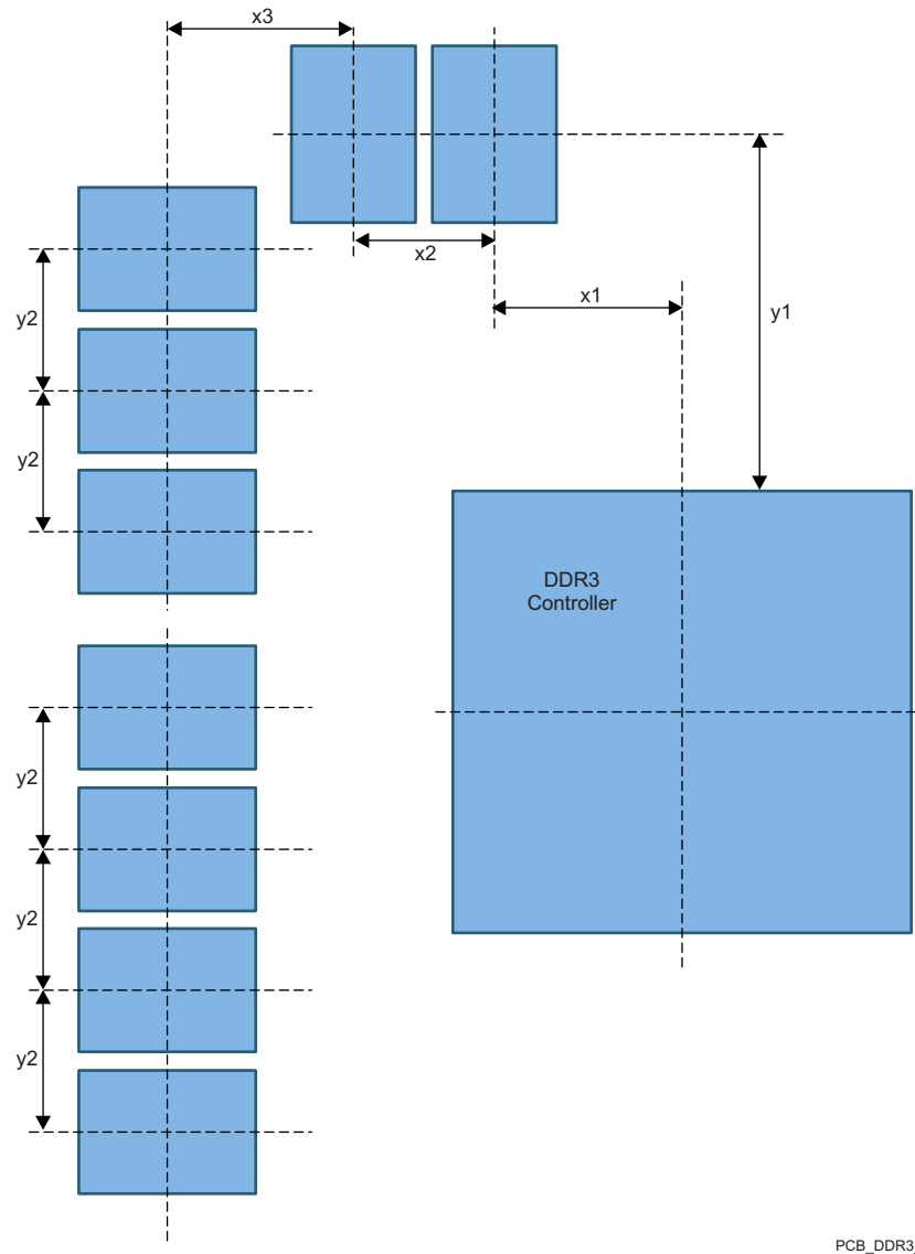
Figure 8-4. Placement Specifications
